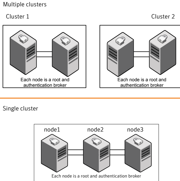
Figure 1-2 Typical configuration of SF Sybase CE clusters in secure mode
