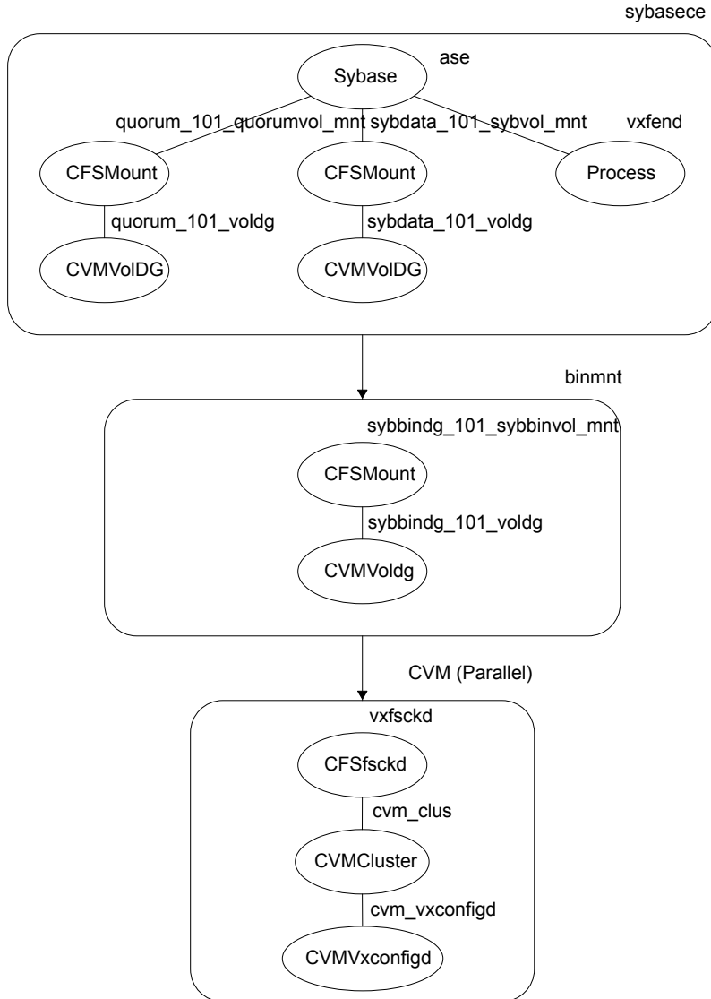
Figure 17-2 Service group dependencies for an SF Sybase CE configuration on shared disk group with CFS
