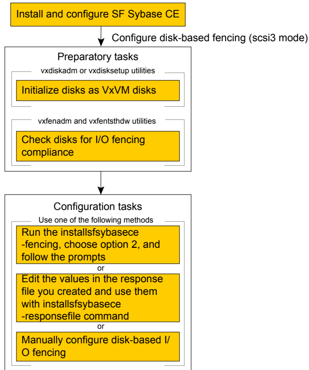
Figure 3-1 Workflow to configure I/O fencing
