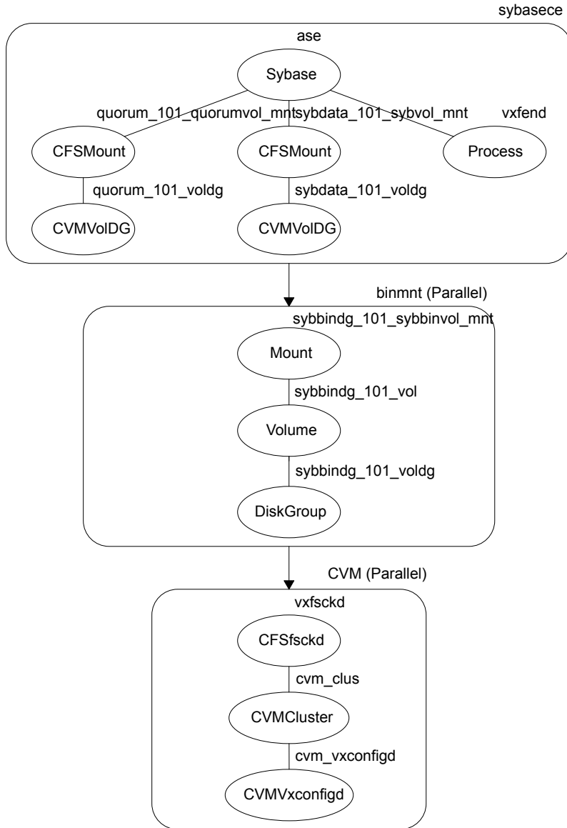
Figure 17-2 displays the service group dependencies for an SF Sybase CE configuration on shared disk group with CFS.
