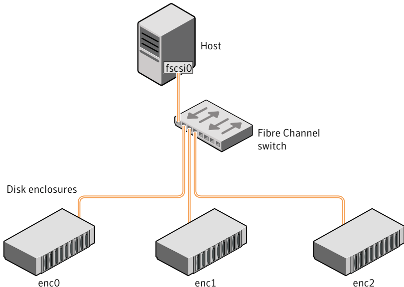
Figure 6-3 Example configuration for disk enclosures connected via a fibre channel switch
