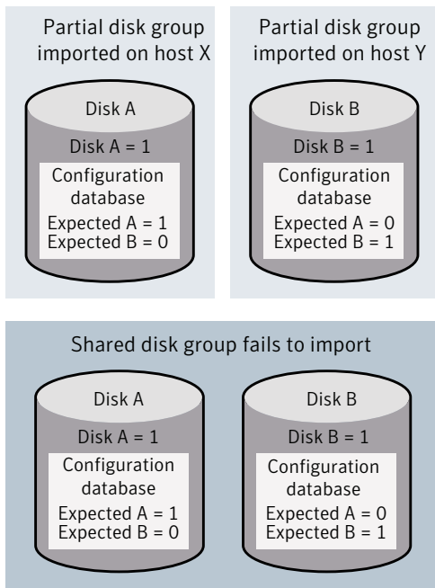
Figure 38-7 Example of a true serial split brain condition that cannot be resolved automatically
