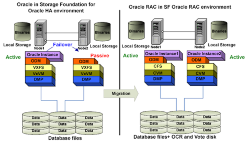
Figure 21-1 Migration from Storage Foundation for Oracle HA to SF Oracle RAC
