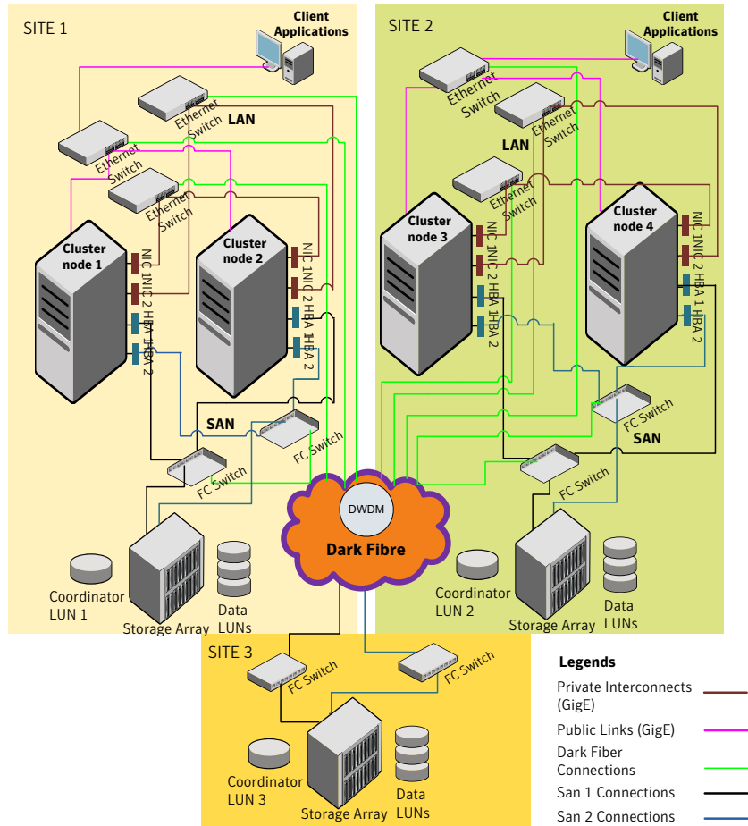
Figure 34-1 Sample SF Oracle RAC configuration
