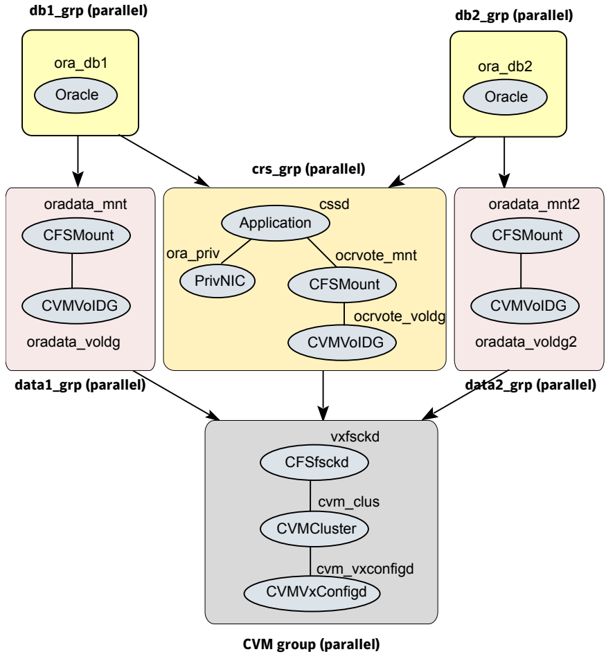
Figure 25-3 Service group configuration with the VCS Oracle agent (alternate configuration)
