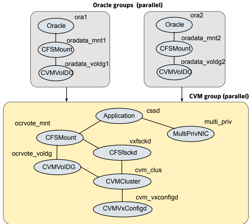
Figure 25-3 illustrates an alternate service group configuration with the VCS Oracle agent.
