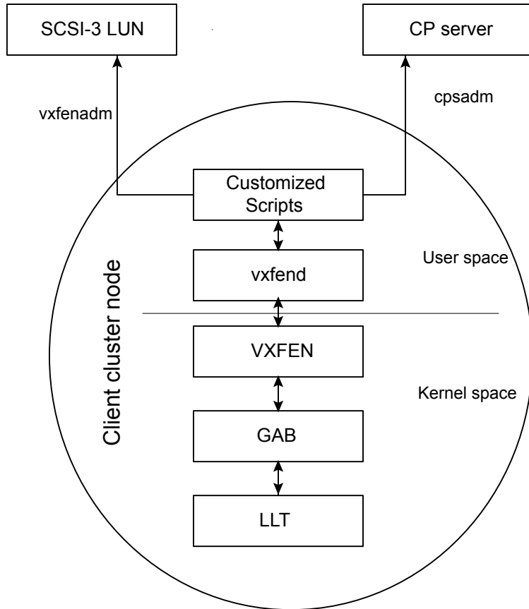
Figure 2-2 Customized fencing
