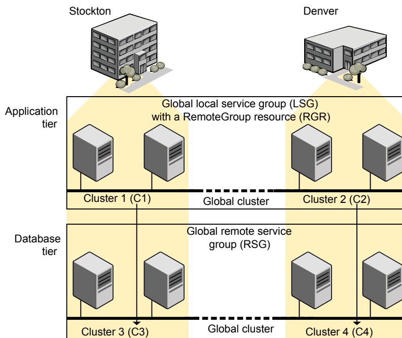
Figure 16-5 A VCS two-tiered globally clustered application and database
