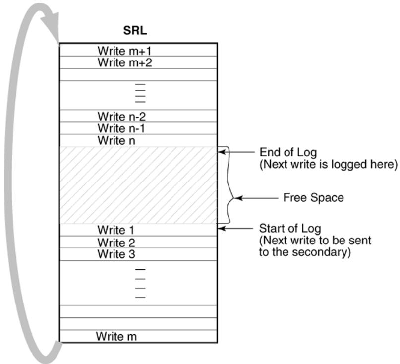
Figure 5-8 Example—How VVR Logs Writes to the SRL
