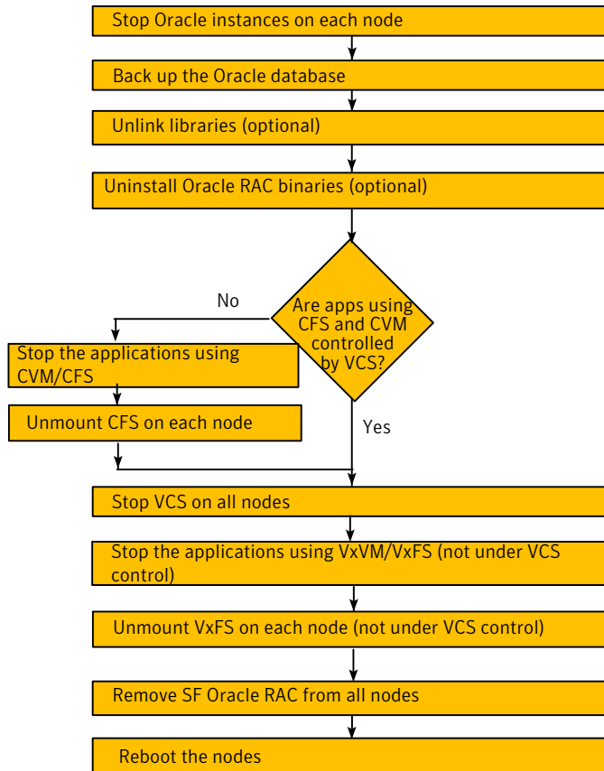
Figure 35-1 SF Oracle RAC uninstallation
