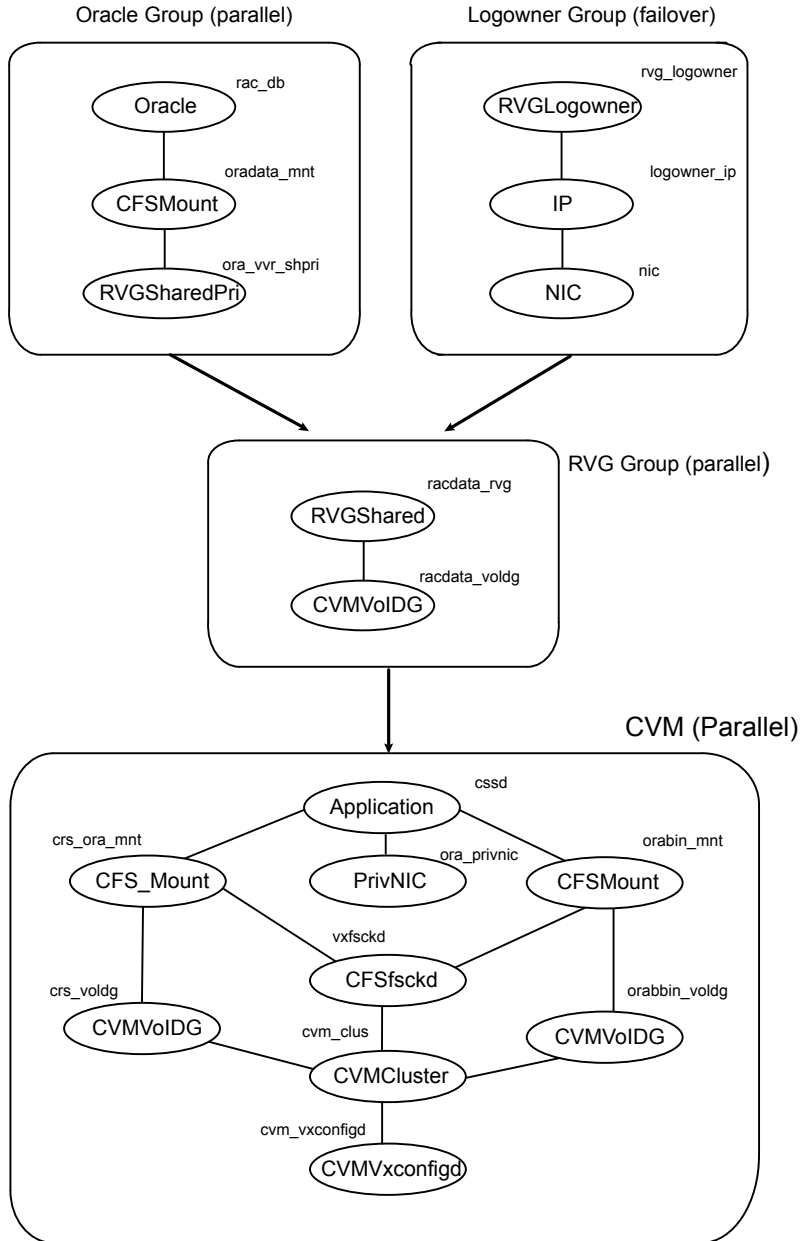
Figure 34-2 Illustration of dependencies after modification for replication of Oracle RAC
