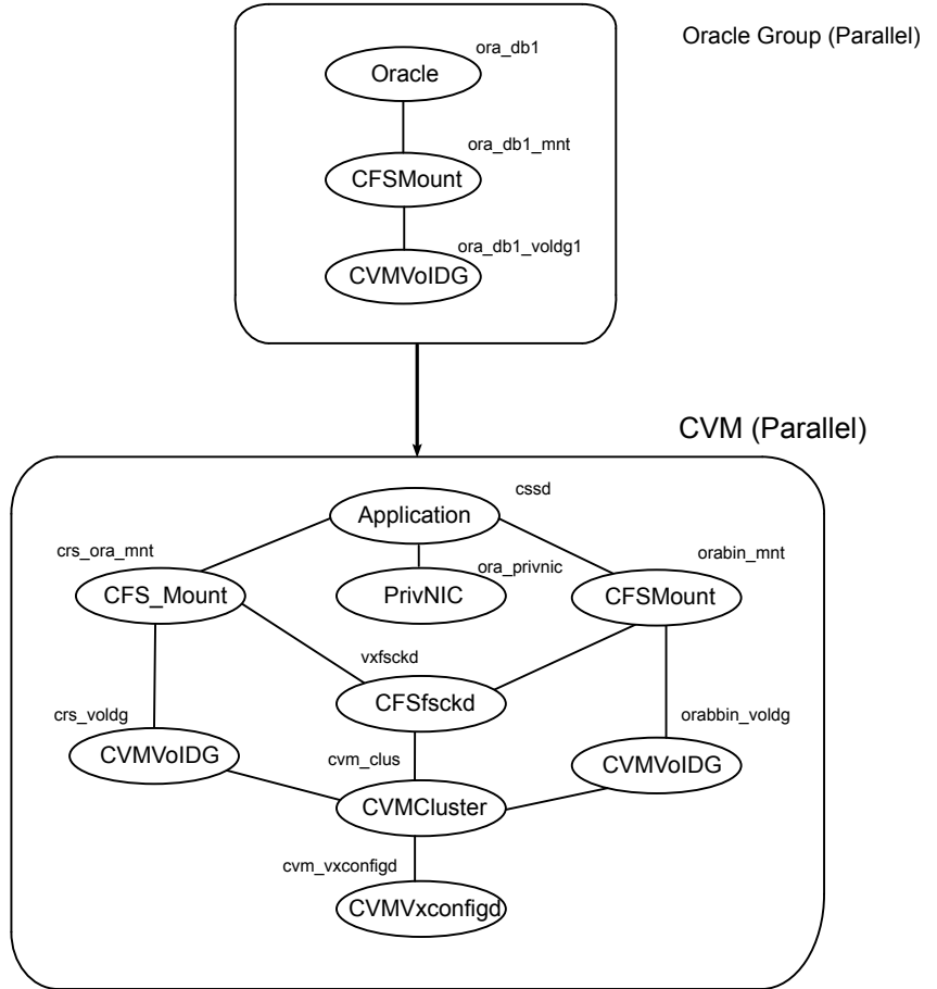
Figure 34-1 Illustration of dependencies before modification for replication
