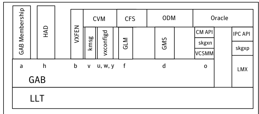
Figure 1-7 Low-level communication
