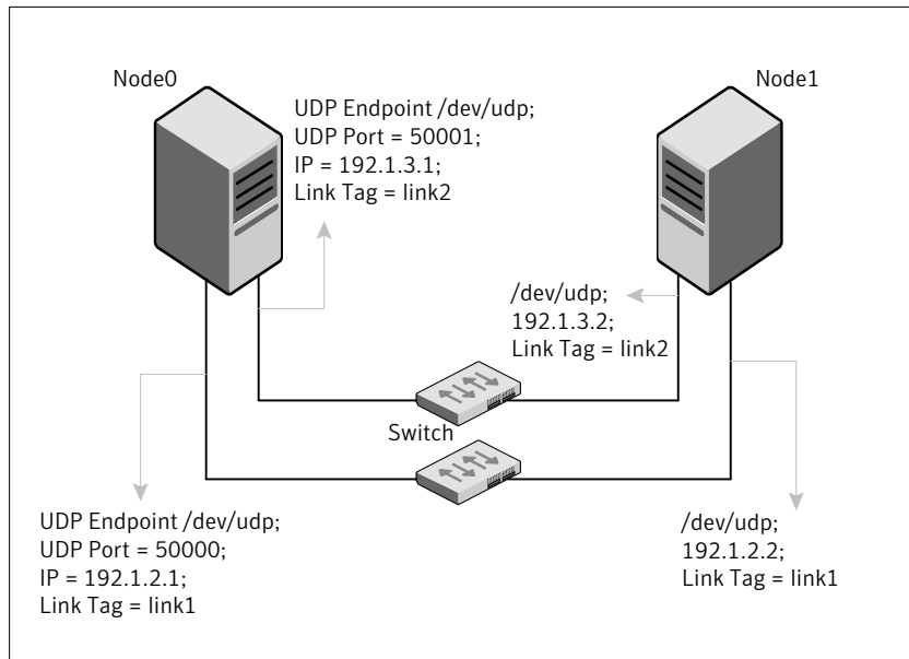
Figure K-1 A typical configuration of direct-attached links that use LLT over UDP
