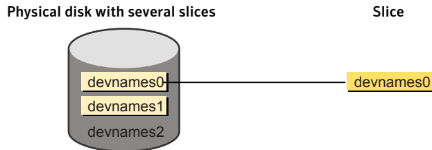
Figure 4-2 Slice example
