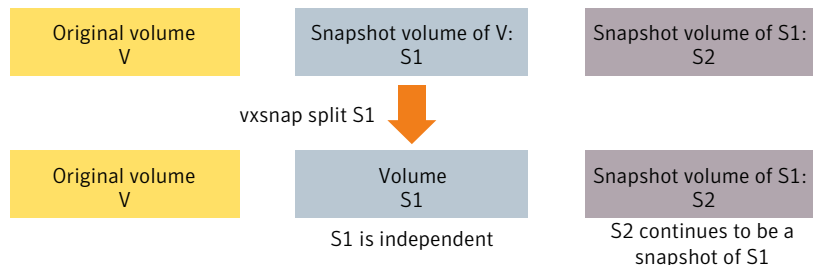
Figure 23-7 Splitting snapshots
