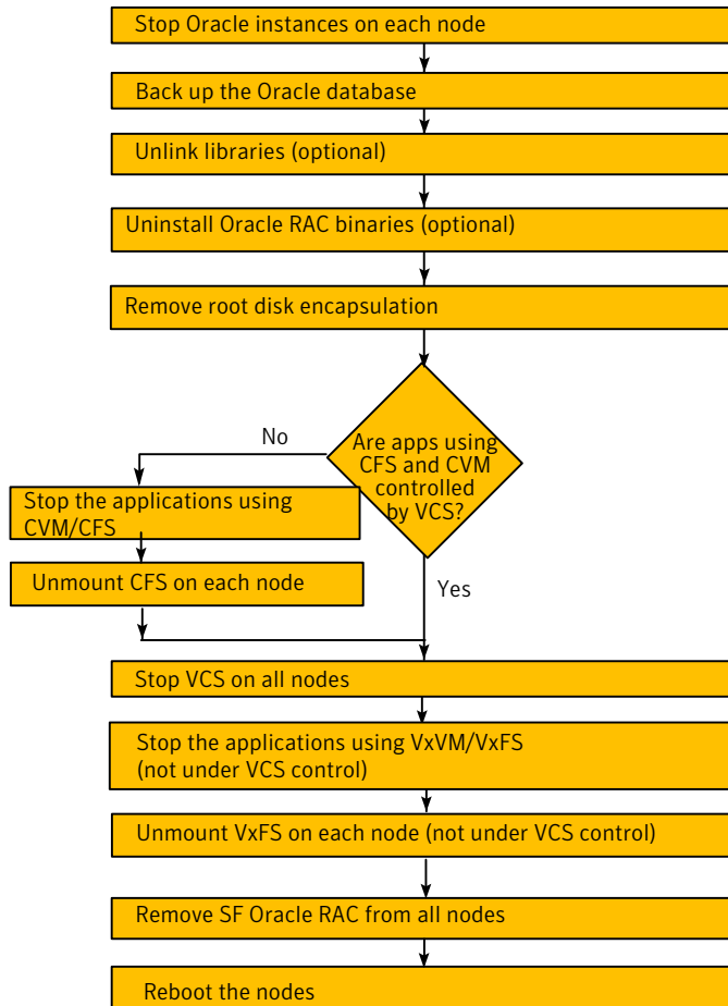
Figure 32-1 SF Oracle RAC uninstallation
