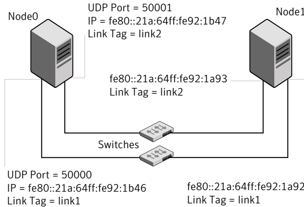
Figure J-3 A typical configuration of direct-attached links that use LLT over UDP
