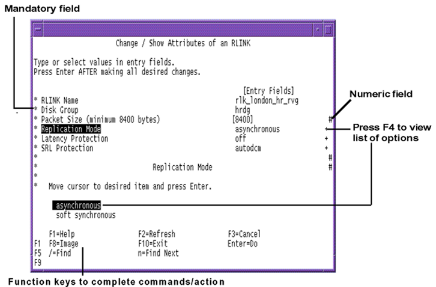
Figure 16-1 Example SMIT screen
