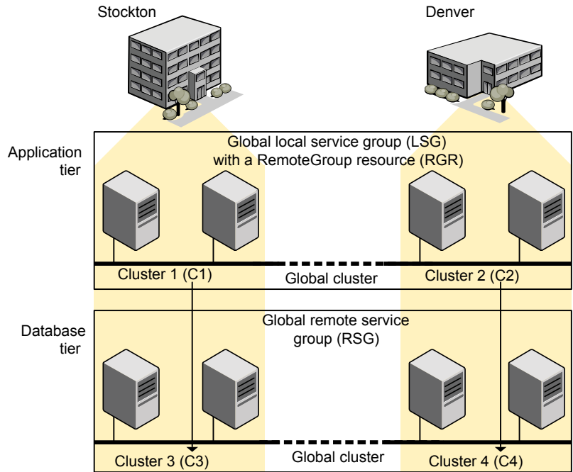
Figure 18-5 A VCS two-tiered globally clustered application and database
